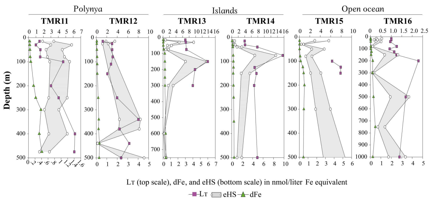
Fig. 2. Combined data for eHS, dFe, and L_T . Individual profiles for stations TMR11 to TMR16 of dFe (green triangle) and total Fe-binding organic ligand ( L_T , purple square) concentrations with an envelope (gray) for eHS, encompassing the maximum and minimum Fe-binding capacities reported for terrestrial International Humic Substances Society (IHSS) standards. Each plot represents one measurement from seawater samples collected in the Mertz glacier polynya (TMR11 and TMR12), downstream of the Balleny islands (TMR13 and TMR14) and in the open ocean near the Balleny islands (TMR15) or the Ross Sea (TMR16).
