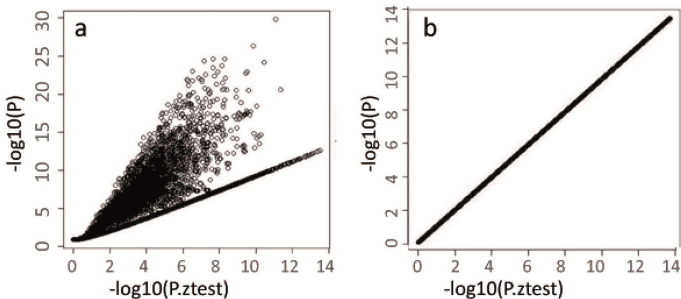
Figure 3. P-Z plot to reveal analytical issues with beta, standard error and P-values
