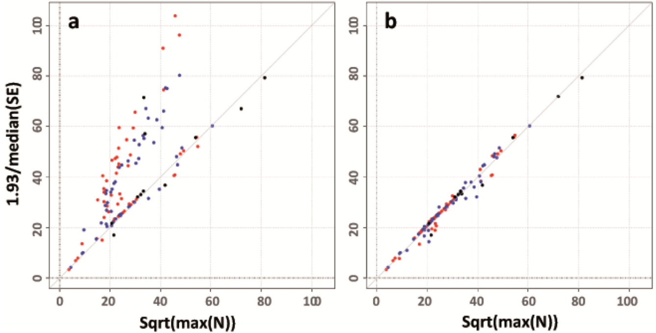
Figure 2. SE-N plots to reveal issues with trait transformations
